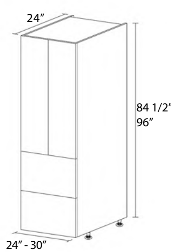
2 DOORS • 2 • 3 SHELVES 2 DRAWERS
