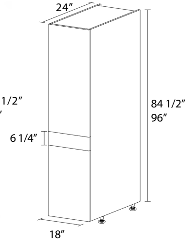
2 DOORS • 3 SHELVES • 4 SHELVES 1 DRAWER R: RIGHT L: LEFT
