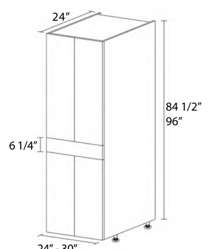
4 DOORS • 3 • 4 SHELVES 1 DRAWER
