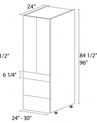
2 DOORS • 2 • 3 SHELVES 3 DRAWERS
